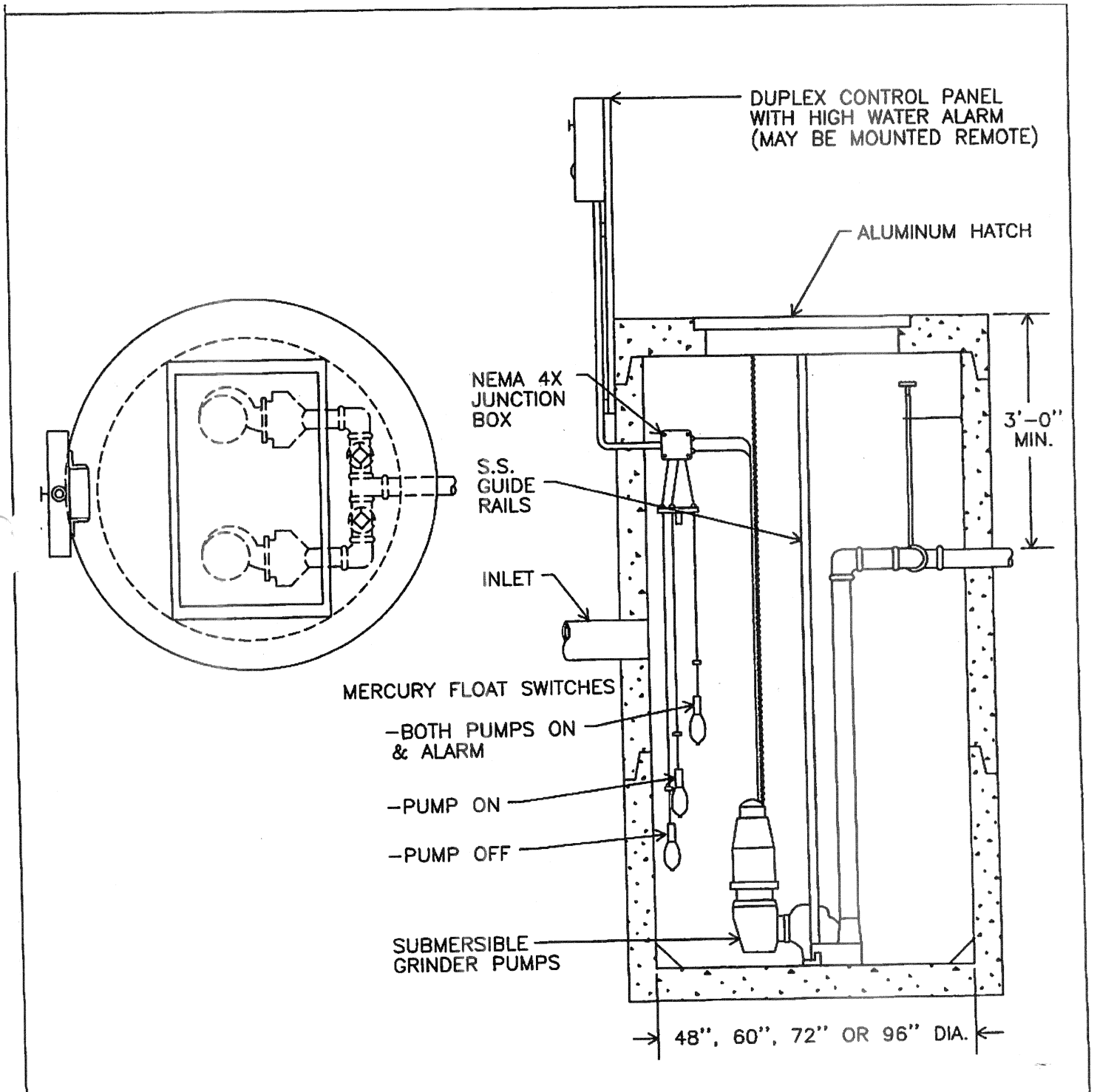
DUPLEX GRINDER PUMP STATION WITH PUMPS ON RAIL SYSTEM
